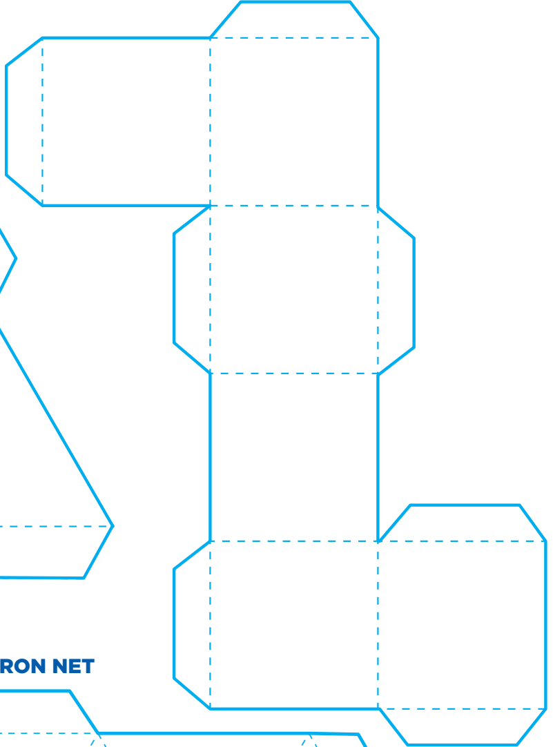
CUBE NET
